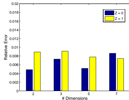
Figure 7: Varying dimensions and skew
