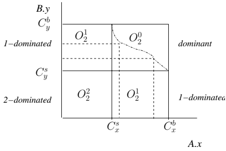
Figure 2: Query Refinement: Phase 2 Every point on the curve in O_2^0 dominates k points
