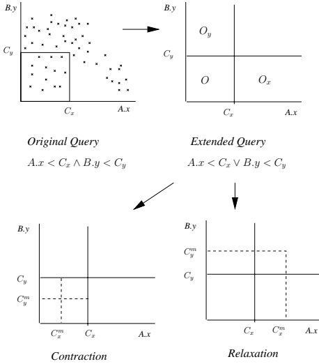
Figure 1: Maximal relaxations and contractions for numeric predicates
