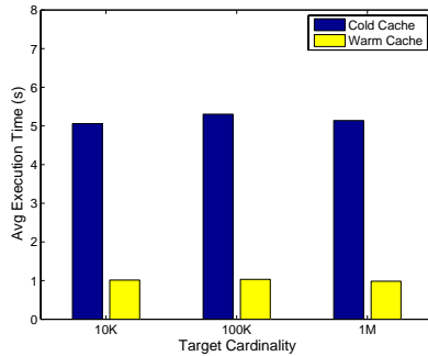
Figure 8: Execution Times
