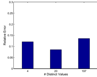
Figure 6: Varying # Distinct Values for relaxation
