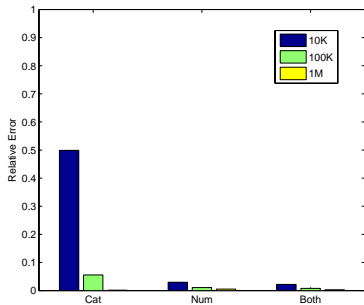
Figure 5: Multiple Query Varying Targets
