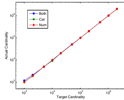
Figure 4: Single Query Varying Target
